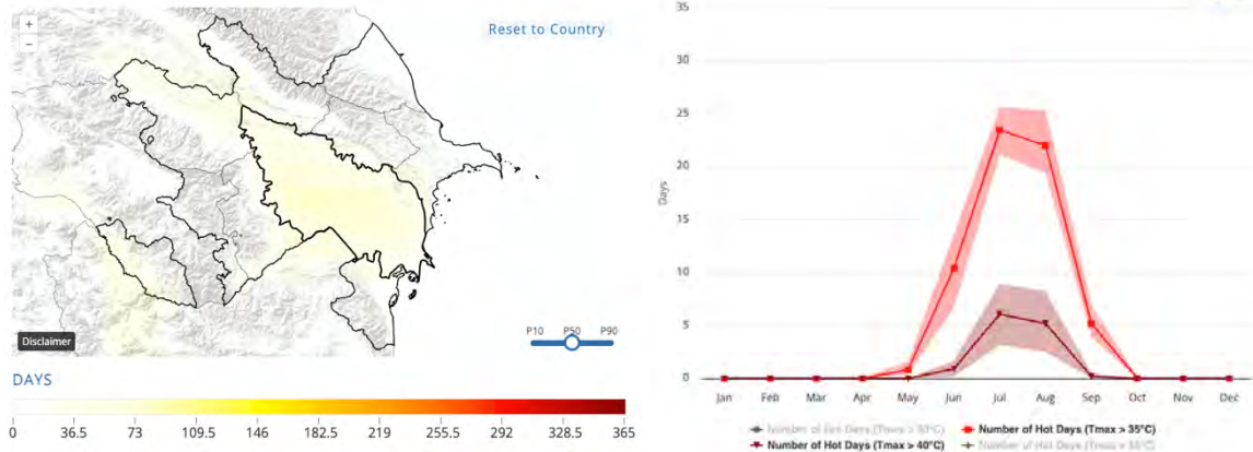
Figure 12 Projected Number of Hot Days ( T_{max} > 35^{\circ}\text{C} ) for the Project Area (2040-2039), SSP2-4.5, 50 th Percentile
