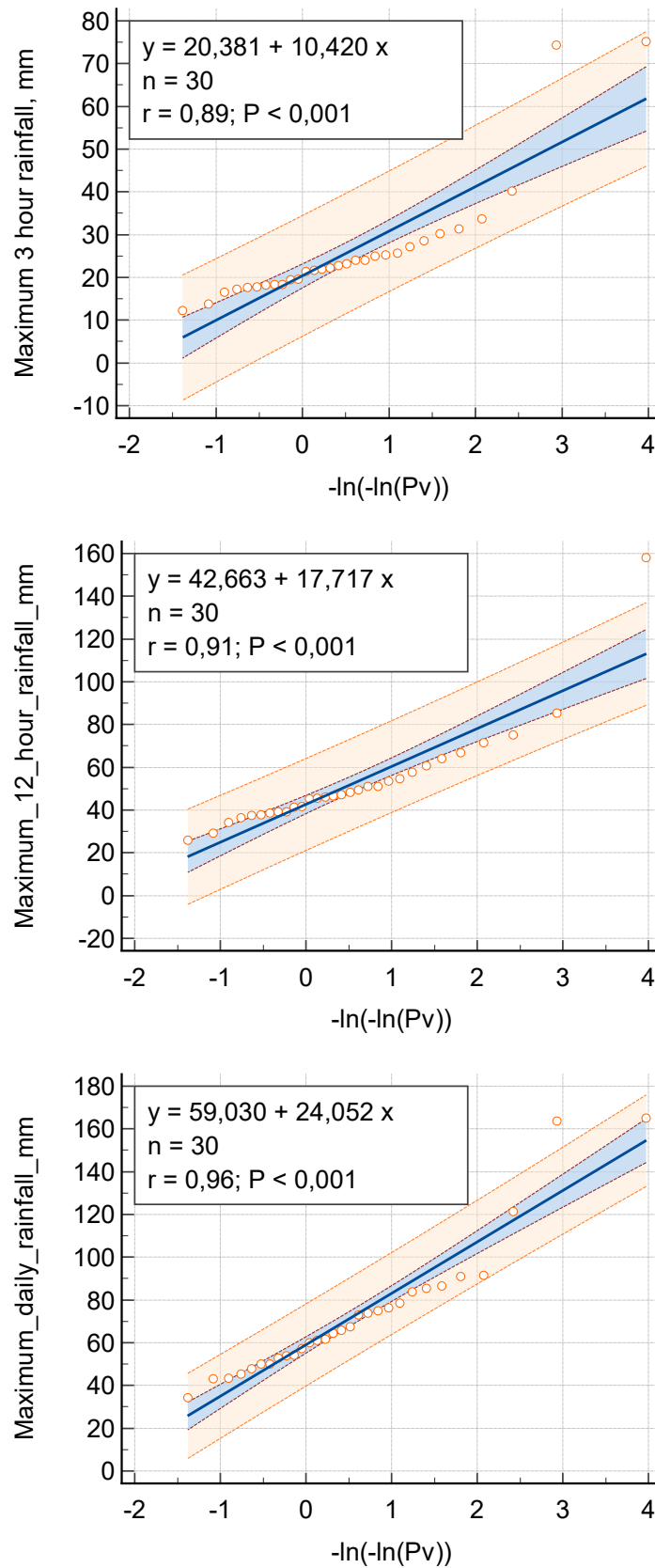
Figure 3.7: Extreme Value Type I distribution of maximums 3-hour, 12 hour and daily rainfall
