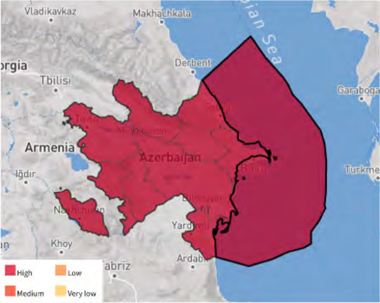
Figure 16 Indication of Projected Wildfire (ThinkHazard, 2024)
