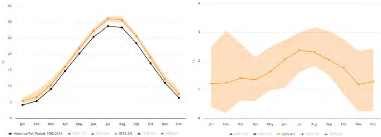
Figure 5 Projected Climatology (Left) and Anomaly (Right) of Average Mean Surface Air Temperature for 2040-2059 (Annual) for the Project Region; (Ref. Period: 1995-2014), SSP2-4.5, Multi-Model Ensemble
