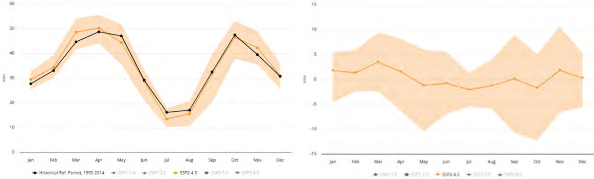
Figure 18 Projected Precipitation Climatology (Left) and Anomaly (Right) for 2020-2039 (Annual) for the Project Region; (Ref. Period: 1995-2014), SSP2-4.5, Multi-Model Ensemble
