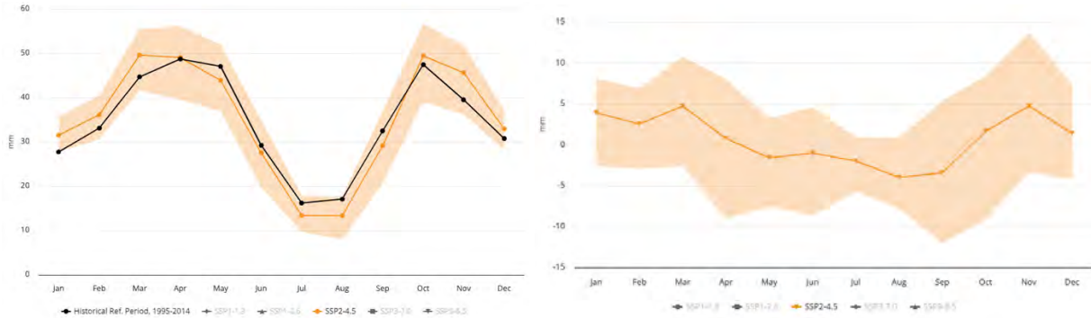
Figure 19 Projected Precipitation Climatology (Left) and Anomaly (Right) for 2040-2059 (Annual) for the Project Region; (Ref. Period: 1995-2014), SSP2-4.5, Multi-Model Ensemble
