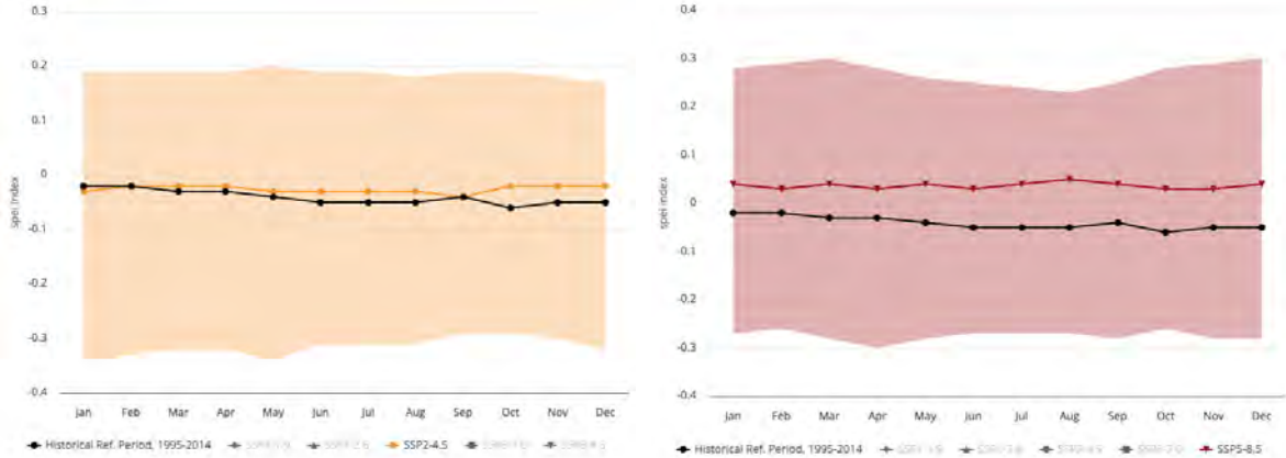
Figure 28 Projected Climatology of Annual SPEI Drought Index for 2020-2039 (Annual) for the Project Region; (Ref. Period: 1995-2014), SSP2-4.5 (Left) SSP5-8.5 (Right), Multi-Model Ensemble
