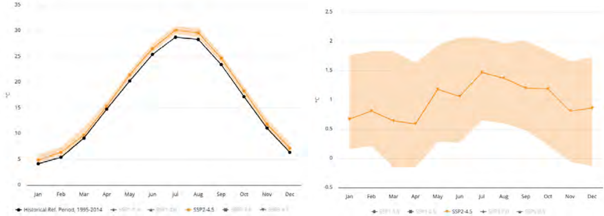
Figure 4 Projected Climatology (Left) and Anomaly (Right) of Average Mean Surface Air Temperature for 2020-2039 (Annual) for the Project Region; (Ref. Period: 1995-2014), SSP2-4.5, Multi-Model Ensemble
